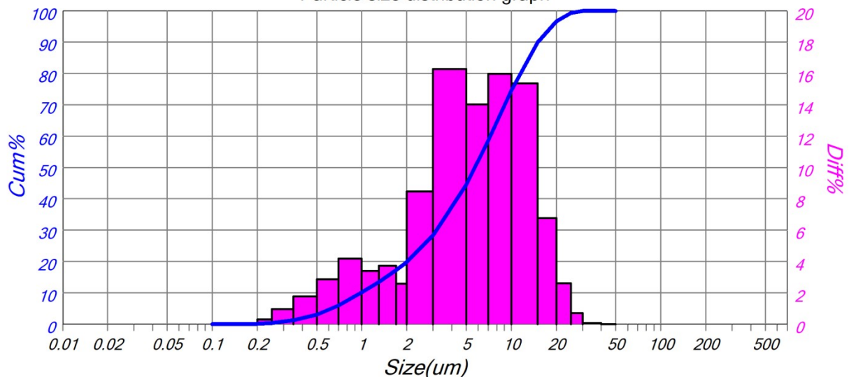
Particle size distribution graph
